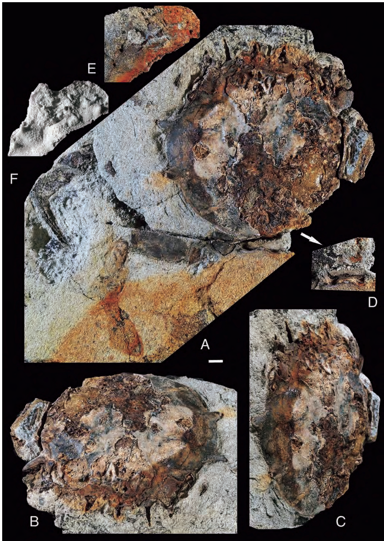
Fig. 1. Orithya eikii , new species. Holotype, MFM9052, Akeyo Formation, Early Miocene. A , dorsal view of carapace and pereopods; B , frontal view of carapace; C , lateral view of carapace; D , outer mold of telson and pleonal somite 6, and pleonal somite 5; E , reversal image of outer mold of anterior region of carapace; F , whitening image coated with ammonium chloride sublimate of latex cast derived from outer mold (Fig. 1E). Scale bar = 5 mm.
