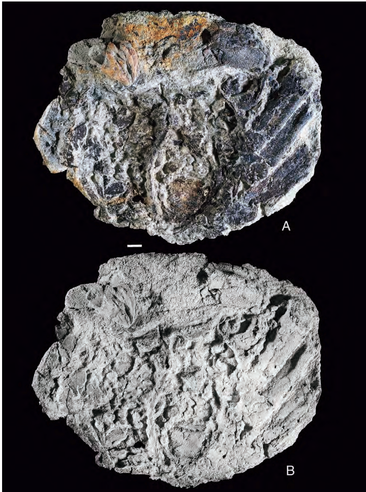
Fig. 3. Orithya eikii , new species. Holotype, MFM9052, Akeyo Formation, Early Miocene. A, B , lateral view of chelipeds and ventral view of thoracic sternum and pereopods 2–5. B is whitening image coated with ammonium chloride sublimate. Scale bar = 5 mm.
